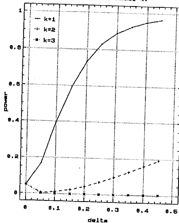
FIGURE 3. Comparison of power functions of G_{40,k} for k = 1, 2 and 3 .
