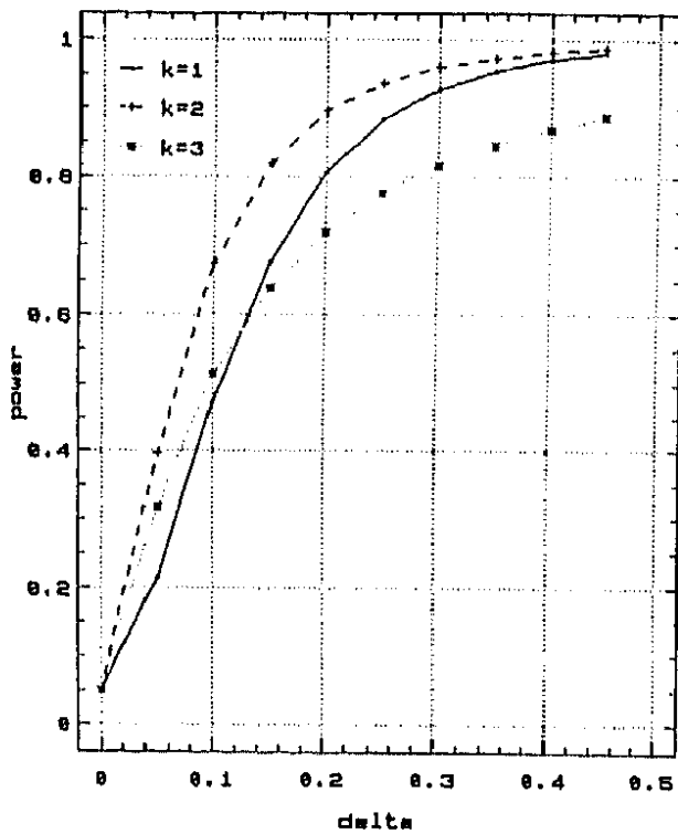
Power comparison of G(n,k) for n=40 and k=1, 2 and 3 . Model 10.
