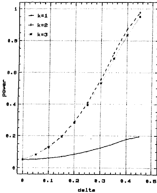
Power comparison of G(n,k) for n=40 and k=1, 2 and 3 . Model 8.
