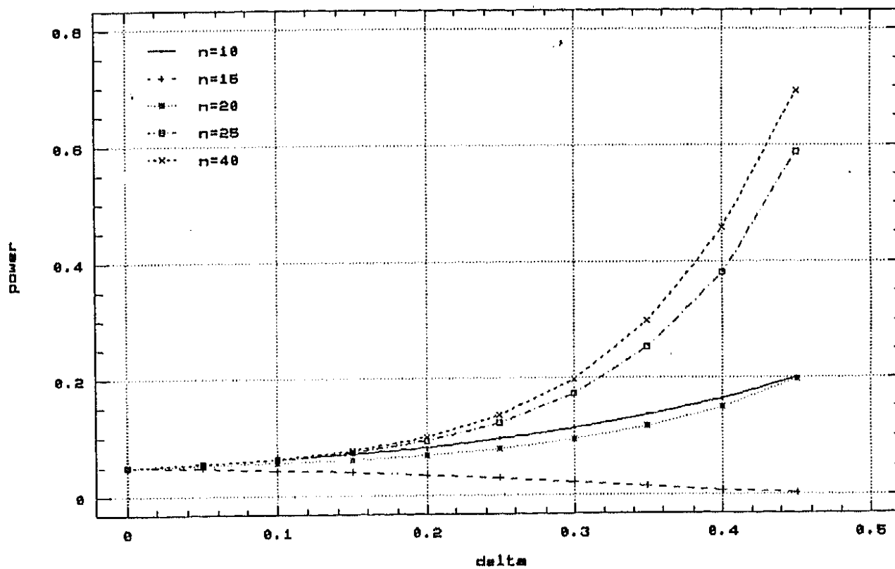
Power function of G(n,k) for k = 1 . Model 7. Left-sided testing
