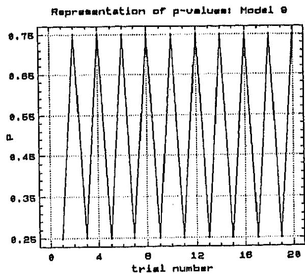
FIGURE 1. Graphical representation of 6 models of nonrandomness
