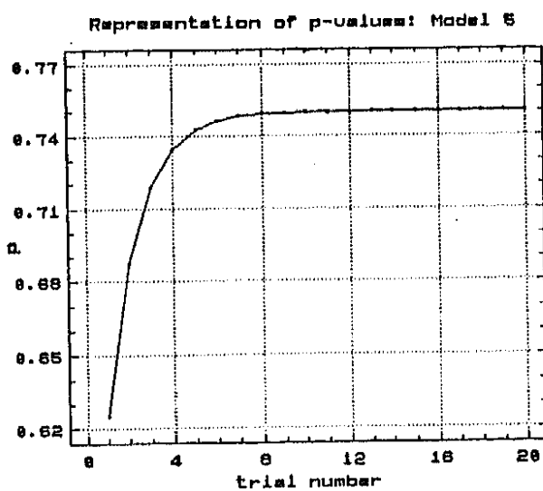
FIGURE 1. Graphical representation of 6 models of nonrandomness
