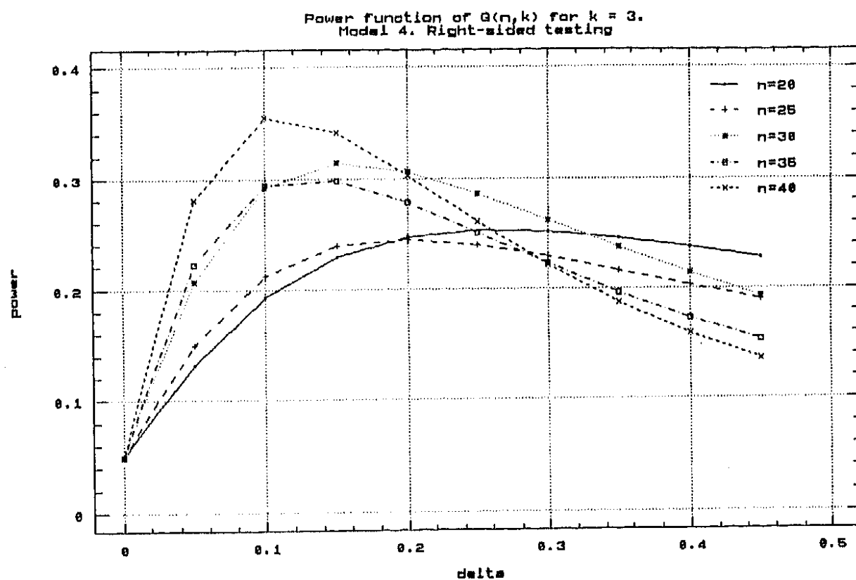
FIGURE 2(c). Power function of G_{n,k} for k = 3 and selected models.
