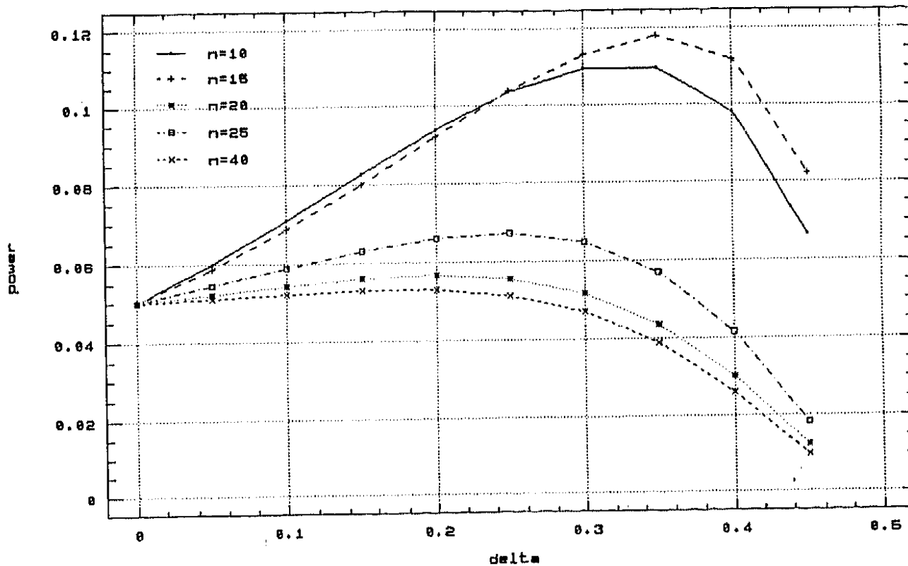
FIGURE 2(a). Power function of G_{n,k} for k = 1 and selected models.
