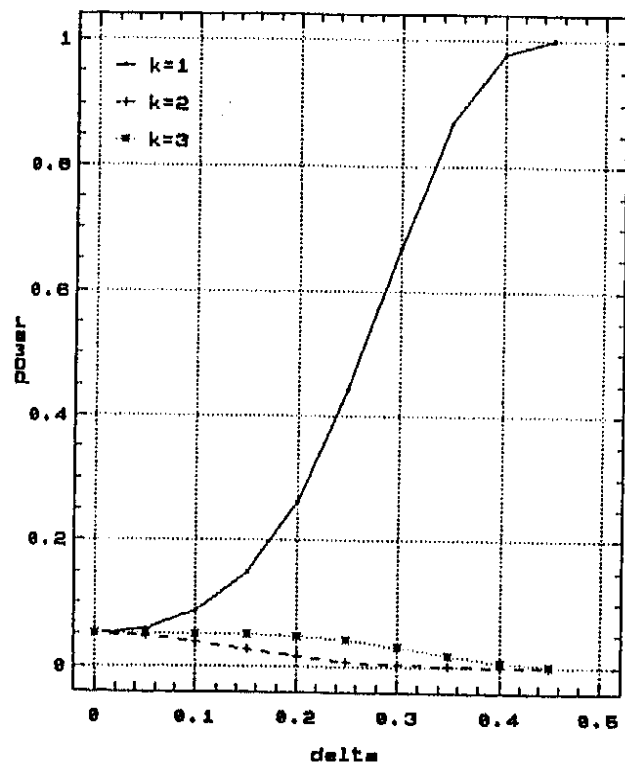
Power comparison of G(n,k) for n=40 and k=1, 2 and 3 . Model 9.
