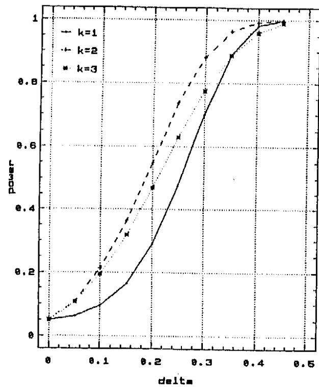
Power comparison of G(n,k) for n=40 and k=1, 2 and 3 . Model 11.
